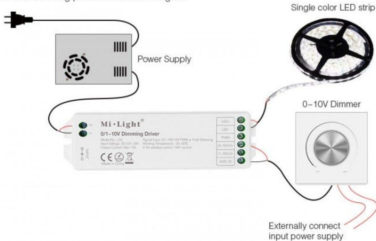
0~10V dimming panel connection diagram
