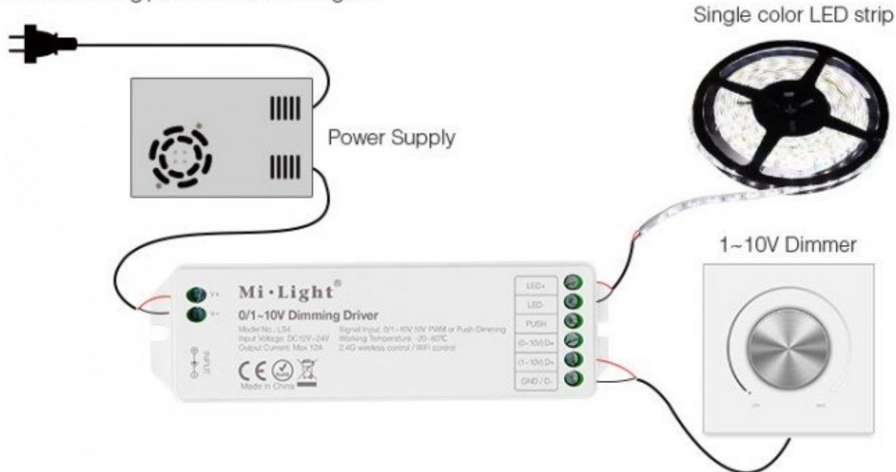
1~10V dimming panel connection diagram
